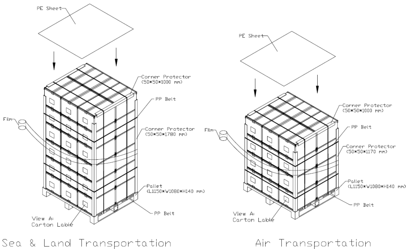
Figure. 7-2 Packing method
